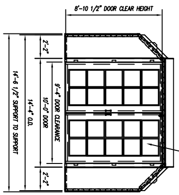
END VIEW FROM BAY END
